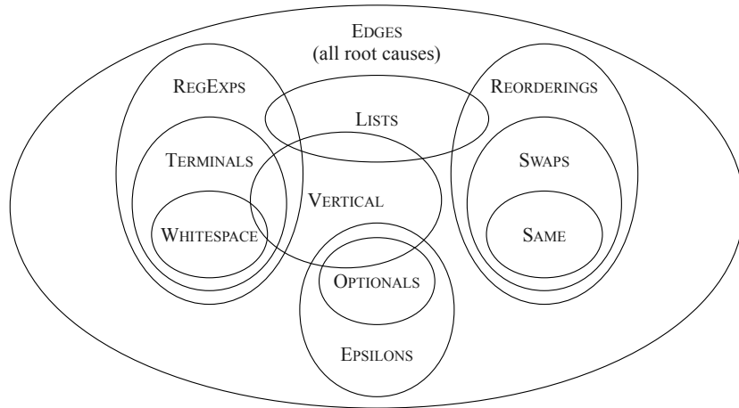
Figure 3. Euler diagram showing the categorization of parse tree differences.
