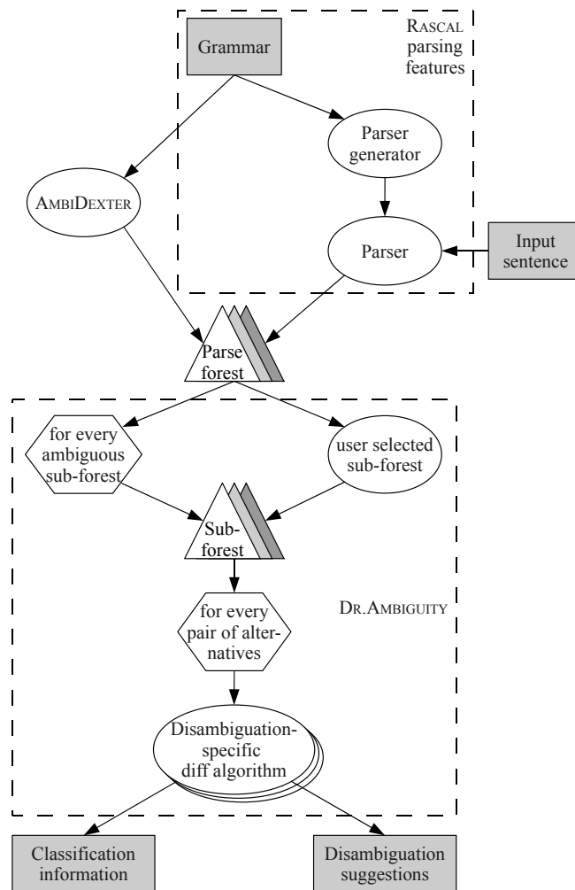
Figure 4. Contextual overview (input/output) of DR. AMBIGUITY.
